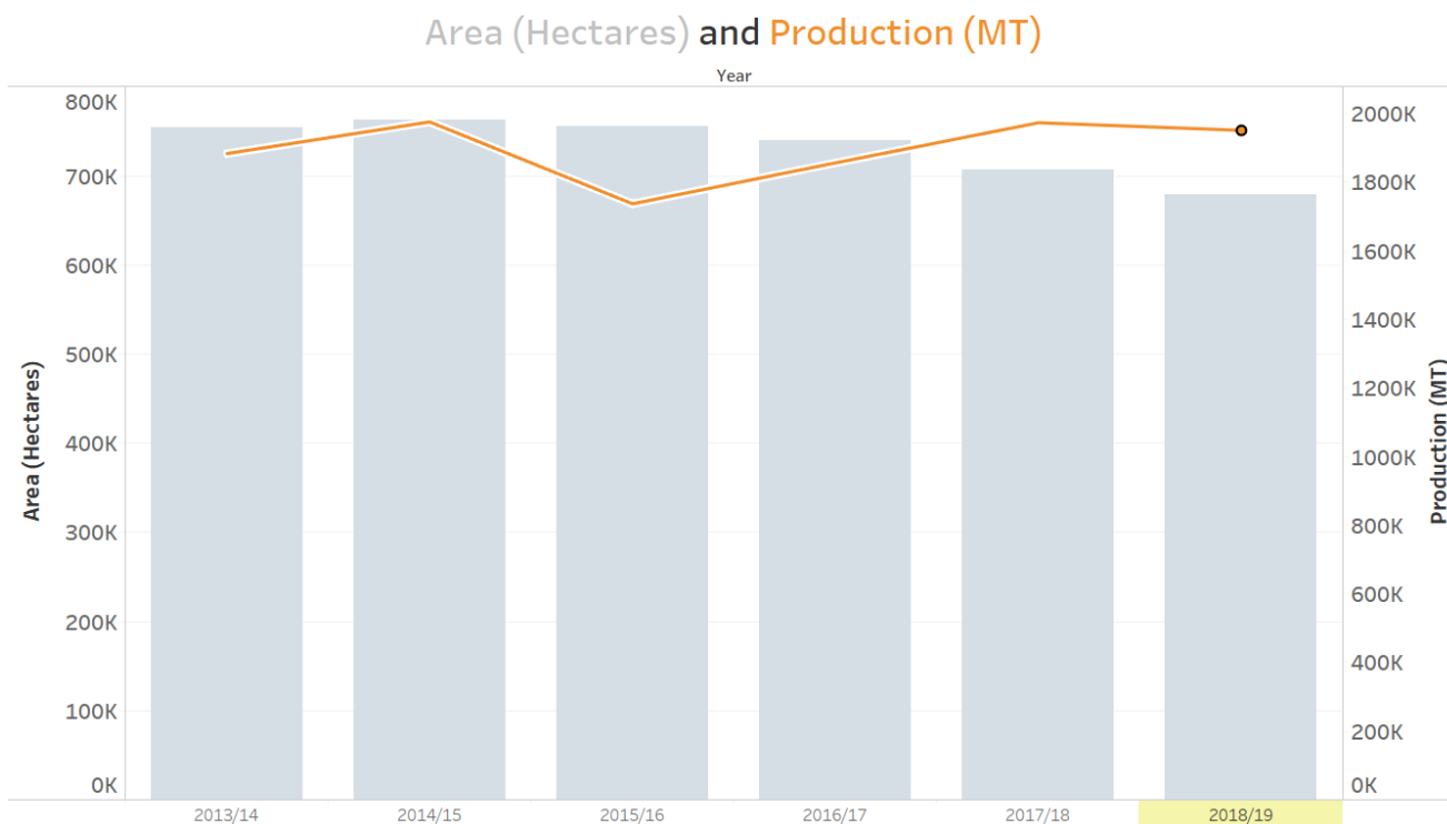
Figure 1: Wheat area, wheat production and CRAFT wheat production forecast for Nepal, 2013-2018 (Source: MoALD; CRAFT)
